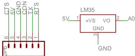
Header for BlueSMiRF gold
