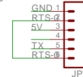
Header for BlueSMiRF mate silver
